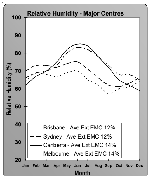
Figure 2 Major centre climates
