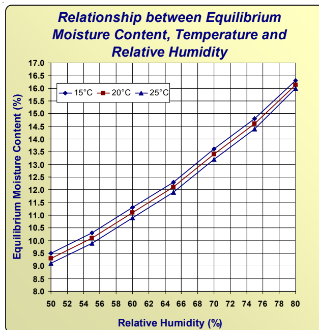
Figure 3 Temperature, RH and EMC
