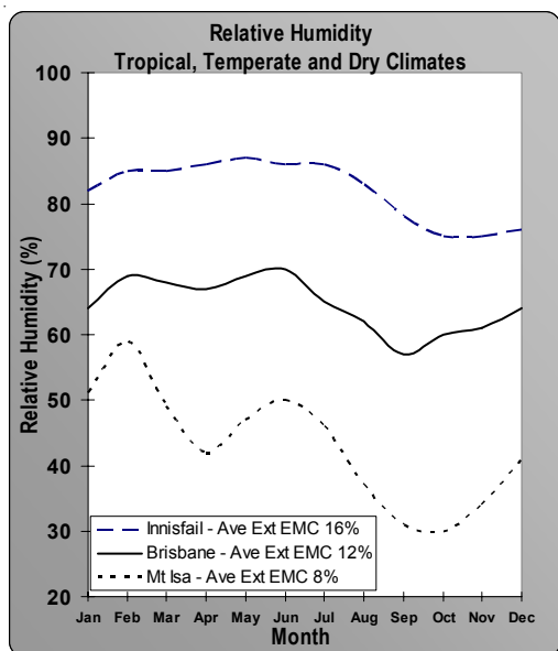
Figure 1 Climatic effects on timber floors
